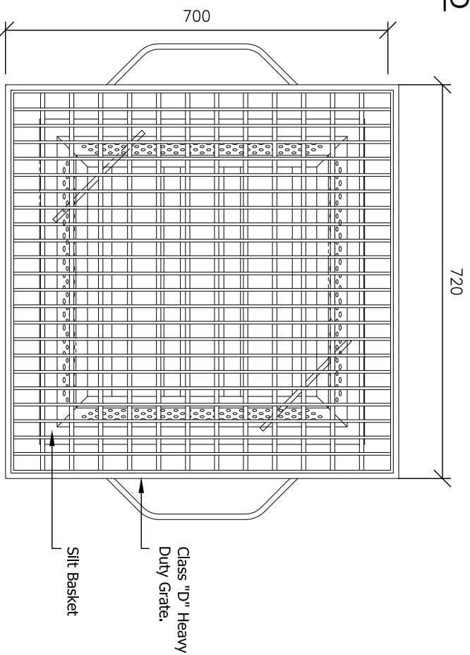
Plan
